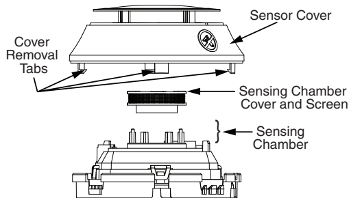
FIGURE 4: CLEANING THE PHOTO/CO DETECTOR
